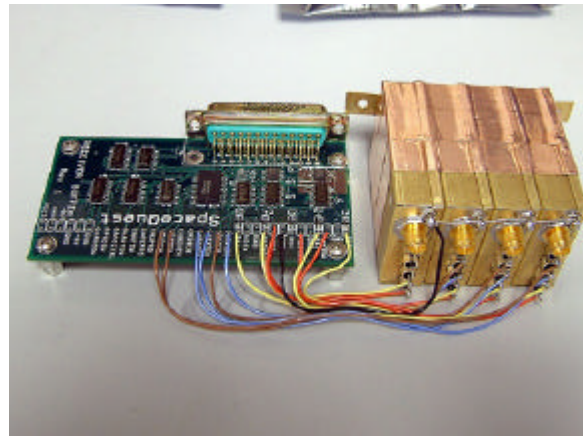
Figure 4: Four VHF Receivers and Interface Board
