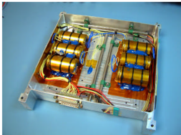
Figure 9: Battery Tray
