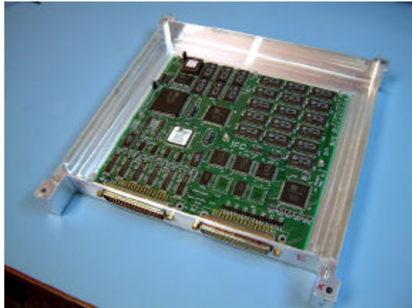
Figure 7: Integrated Flight Computer
