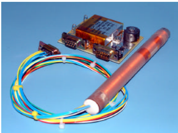
Figure 11: Active Magnetic Attitude Control
