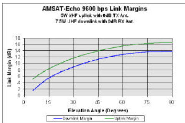
Figure 6: Mode V/U Link Margin Graph
